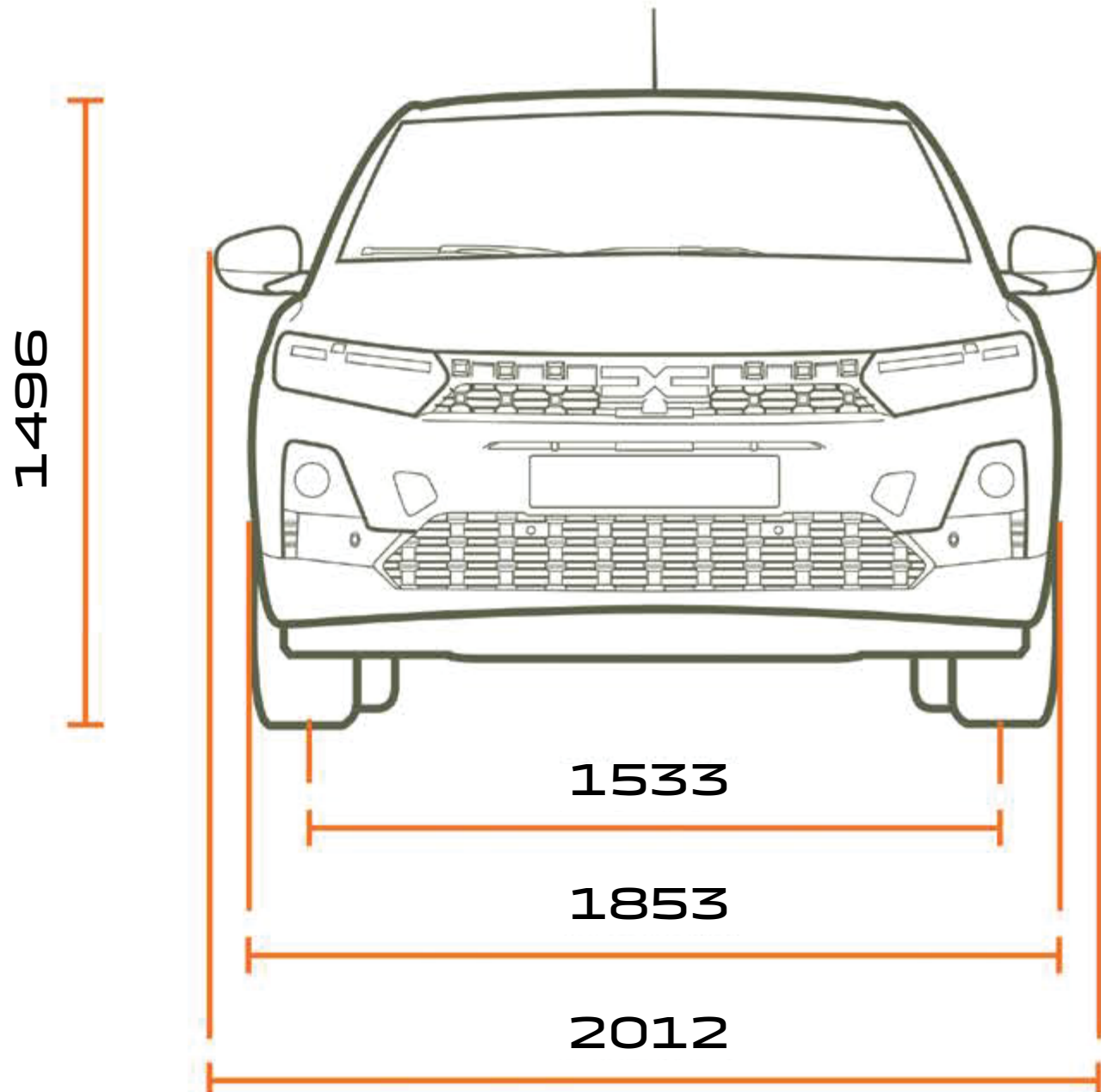
FRONT VIEW
